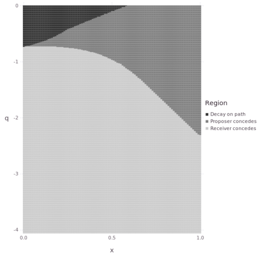
(a) Uniform on [0, 2] .
