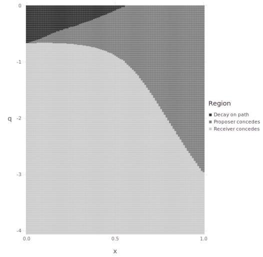
(b) Lognormal ( \mu = -0.5, \sigma = 1.0 )
