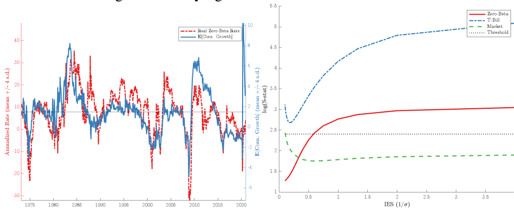
Figure 20: VaryingBetas: Results with Linear Betas
