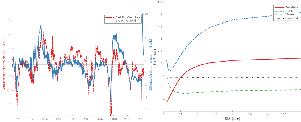
Figure 13: WithConsSigma5: Results with with Consumption Factor, \sigma = 5
