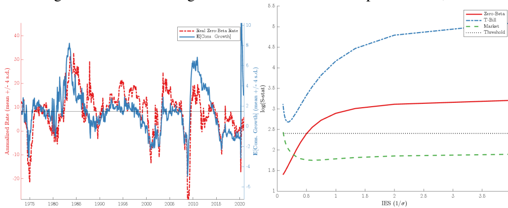
Figure 12: WithConsSigma1: Results with Consumption Factor, \sigma = 1
