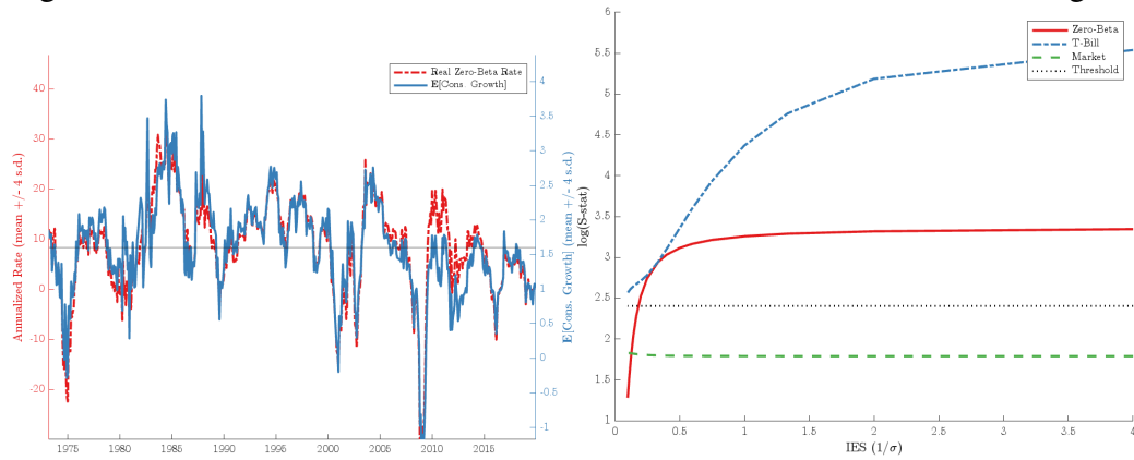
Figure 23: InformativeFactors: Results with “Informative Factors,” Excluding 2020
