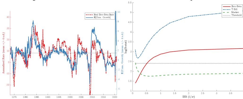
Figure 11: LinearCons: Results with a Linear Consumption Factor
